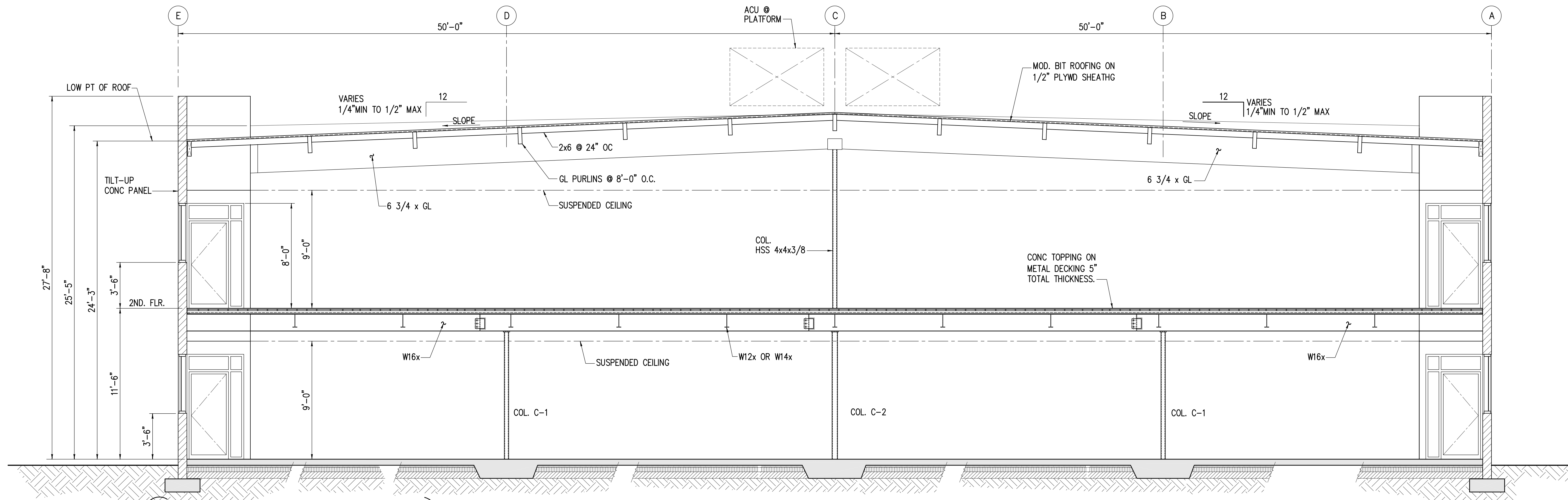
B S-4 BUILDING SECTION SCALE: 1/4"=1'-0"
