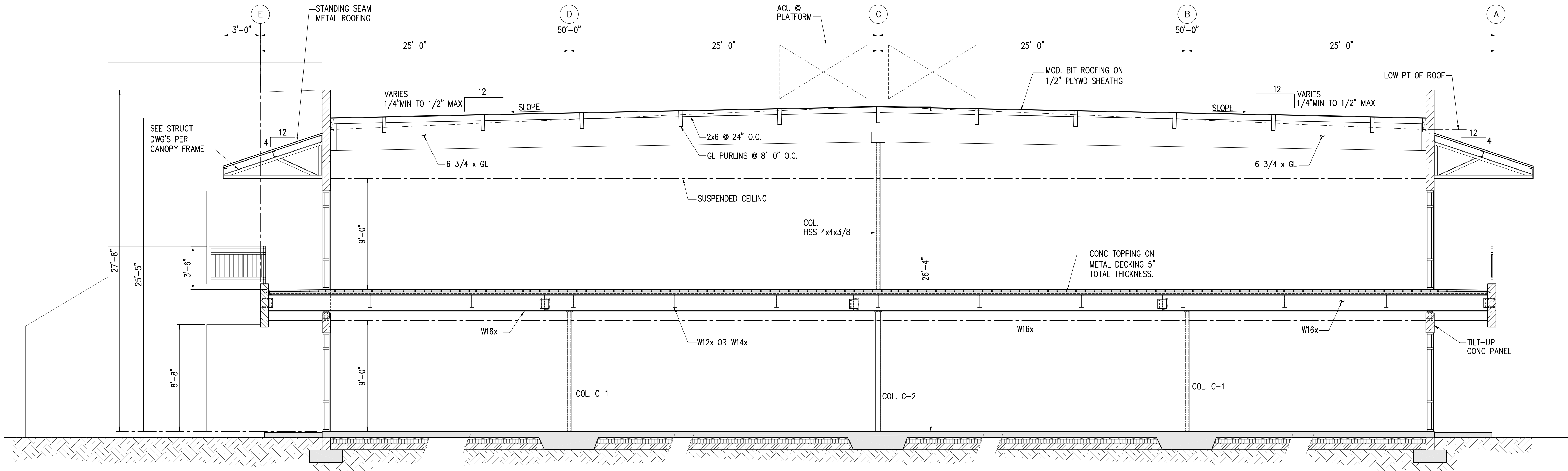
A S-4 BUILDING SECTION SCALE: 1/4"=1'-0"
